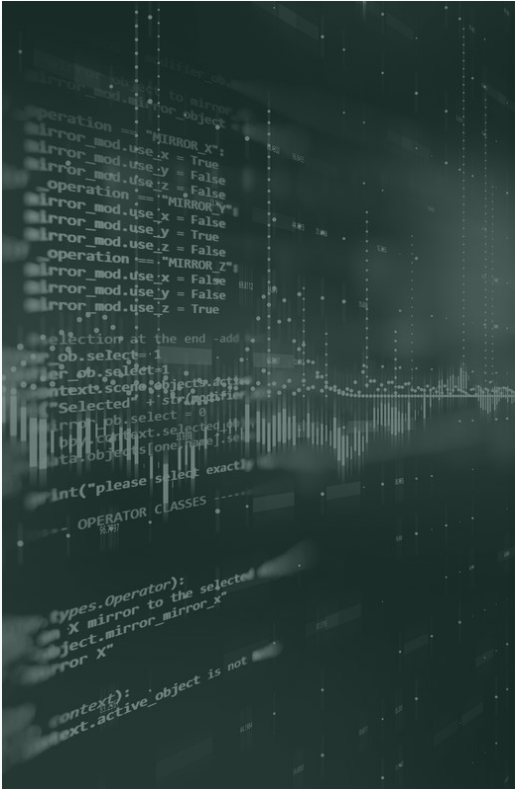
Software
